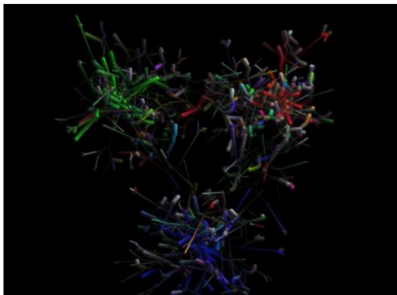
Figure 1: Physical vacuum fluctuations
